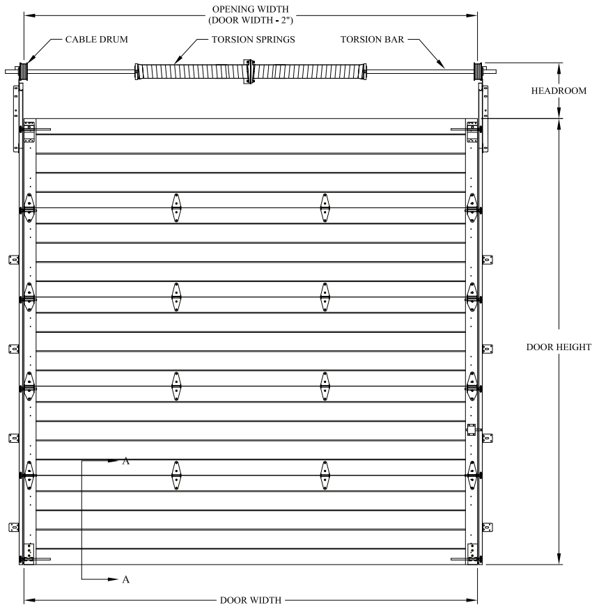
INTERIOR ELEVATION
