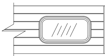
26" x 13 1/2" DOUBLE PANE INSULATED PLEXI-GLASS
