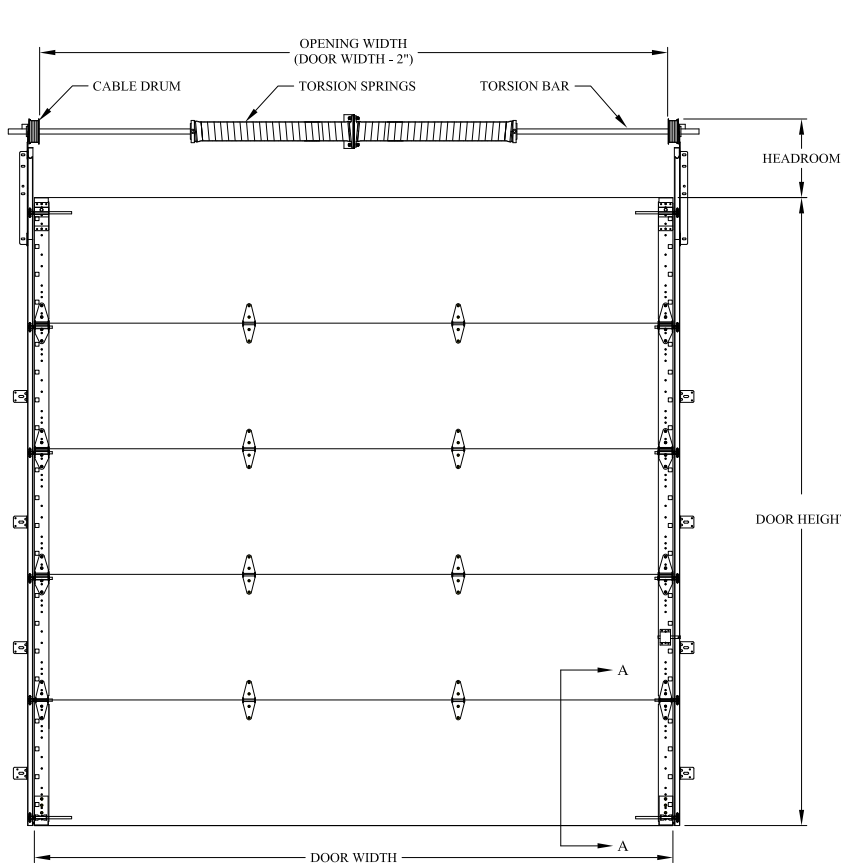
INTERIOR ELEVATION
