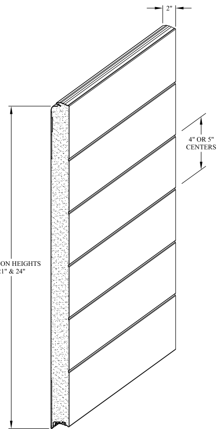
ISOMETRIC PROFILE
