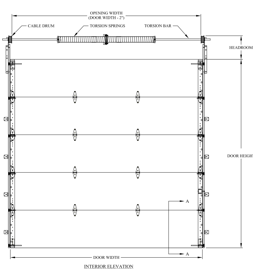
INTERIOR ELEVATION
