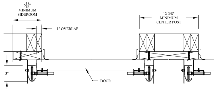
COMMERCIAL 3" TAPERED CONTINUOUS ANGLE MOUNT TO WOOD JAMB DETAIL
