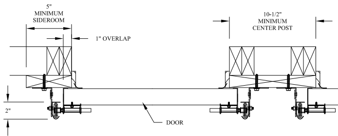
COMMERCIAL 2" CONTINUOUS ANGLE MOUNT TO WOOD JAMB DETAIL
