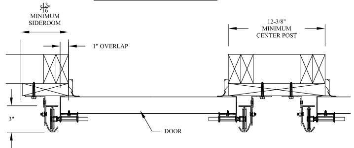
COMMERCIAL 3" CONTINUOUS ANGLE MOUNT TO WOOD JAMB DETAIL
