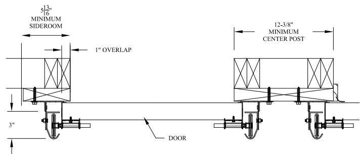
COMMERCIAL 3" REVERSE ANGLE MOUNT WITH JAMB BRACKET ATTACHMENT TO WOOD JAMB DETAIL
