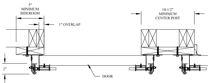
COMMERCIAL 2" REVERSE ANGLE MOUNT WITH JAMB BRACKET ATTACHMENT TO WOOD JAMB DETAIL
