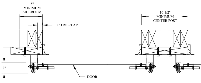
COMMERCIAL 2" BRACKET MOUNT TO WOOD JAMB DETAIL
