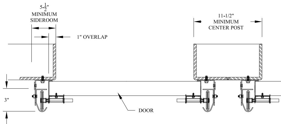
COMMERCIAL 3" REVERSE ANGLE MOUNT TO STEEL JAMB DETAIL
