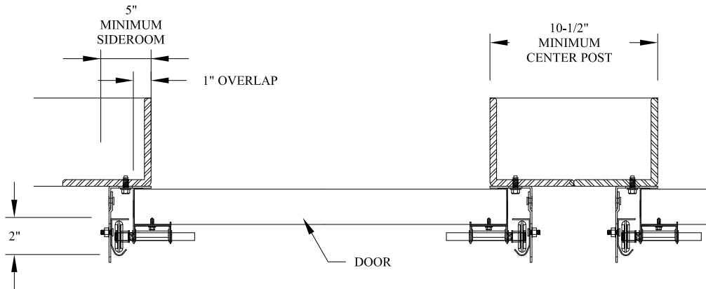
COMMERCIAL 2" REVERSE ANGLE MOUNT TO STEEL JAMB DETAIL
