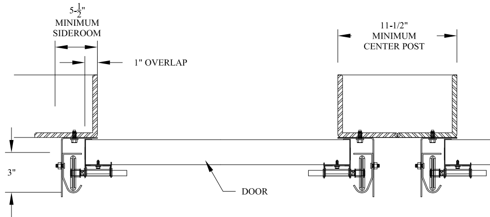
COMMERCIAL 3" TAPERED REVERSE ANGLE MOUNT TO STEEL JAMB DETAIL
