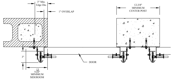
COMMERCIAL 3" CONTINUOUS ANGLE MOUNT TO CONCRETE/MASONRY JAMB DETAIL
