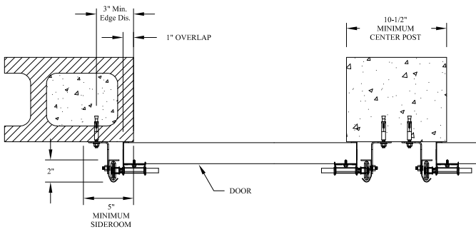
COMMERCIAL 2" BRACKET MOUNT TO CONCRETE/MASONRY JAMB DETAIL
