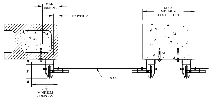
COMMERCIAL 3" REVERSE ANGLE MOUNT WITH JAMB BRACKET ATTACHMENT TO CONCRETE/MASONRY JAMB DETAIL
