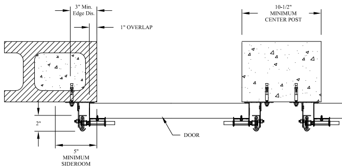
COMMERCIAL 2" REVERSE ANGLE MOUNT WITH JAMB BRACKET ATTACHMENT TO CONCRETE/MASONRY JAMB DETAIL
