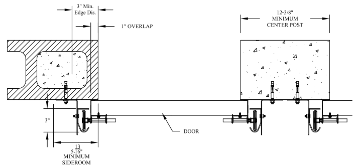
COMMERCIAL 3" TAPERED CONTINUOUS ANGLE MOUNT TO CONCRETE/MASONRY JAMB DETAIL
