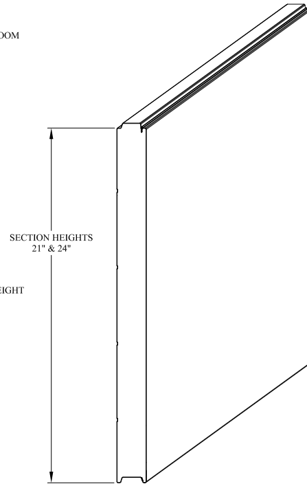
ISOMETRIC PROFILE
