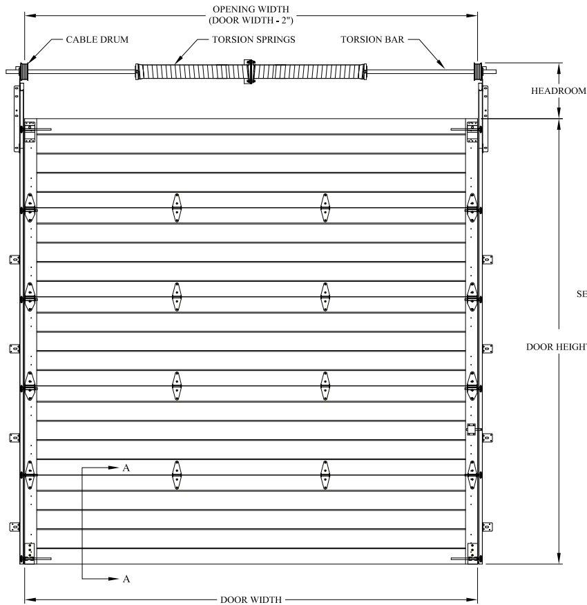
INTERIOR ELEVATION
